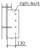
DETAIL I
