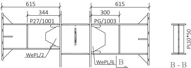
DETAIL B
