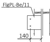
DETAIL_G
