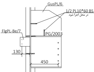
DETAIL H
