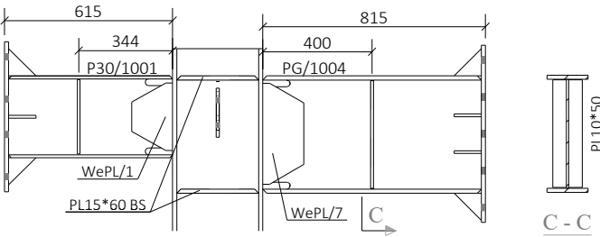
DETAIL C
