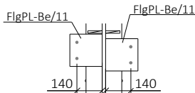
DETAIL G
