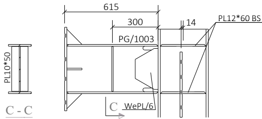
DETAIL C
