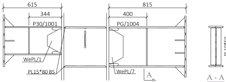
DETAIL A
